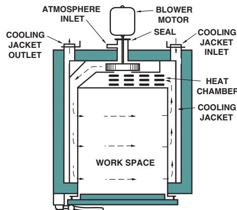
Circulation Diagram (Top View)
